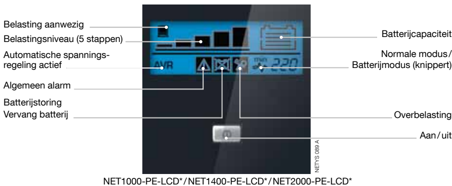
NET1000-PE-LCD*/NET1400-PE-LCD*/NET2000-PE-LCD*
